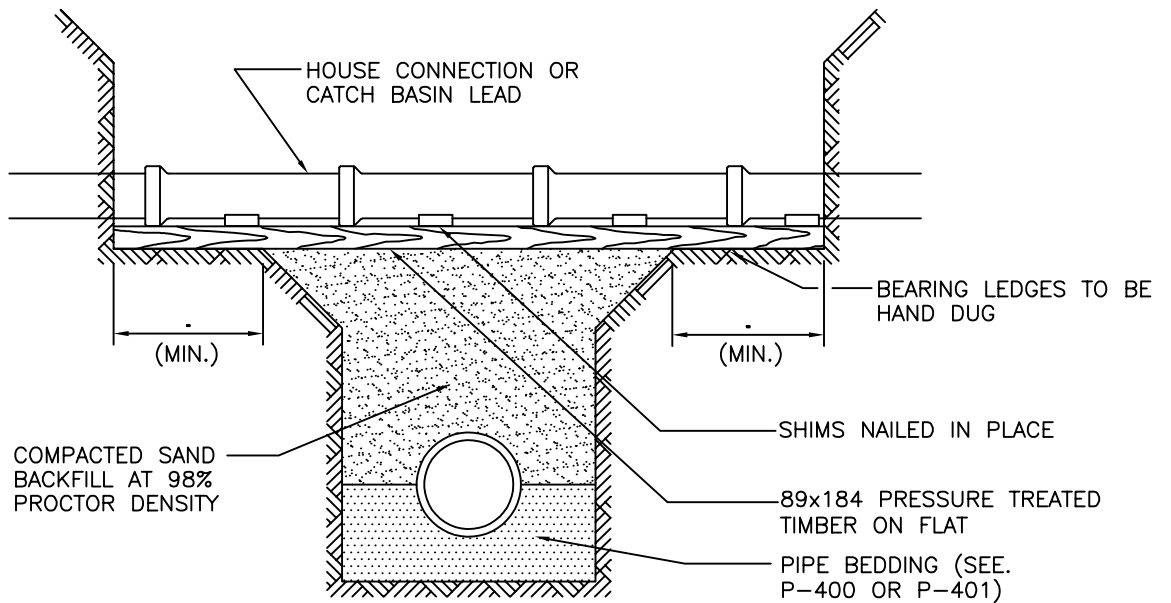
DETAIL "A"
