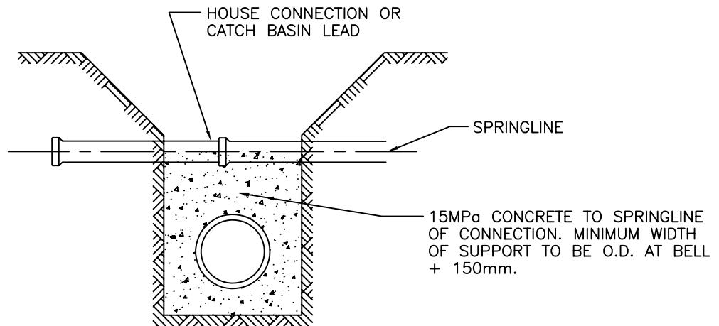
DETAIL "B"
