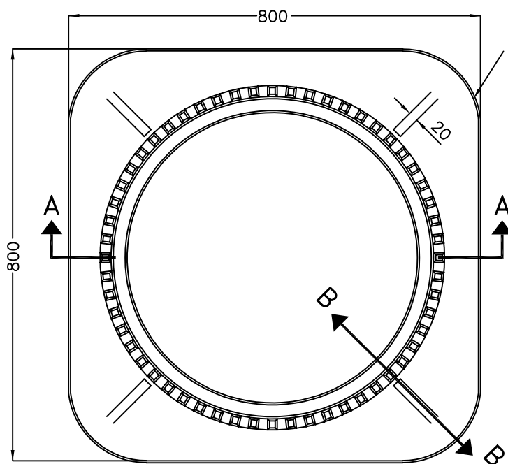
FRAME PLAN
