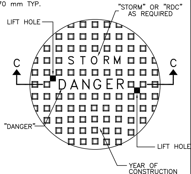
COVER PLAN
