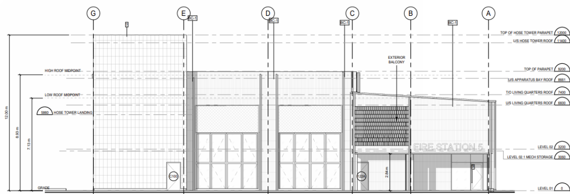
EAST ELEVATION (FLANKAGE)
