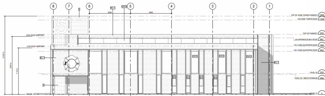
NORTH ELEVATION (FRONT)
