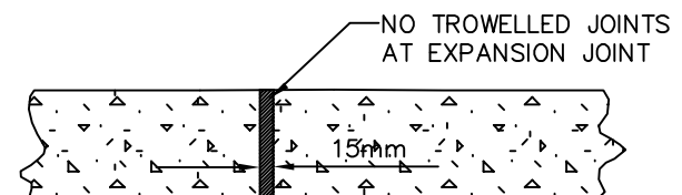
SECTION B-B EXPANSION JOINT DETAIL
