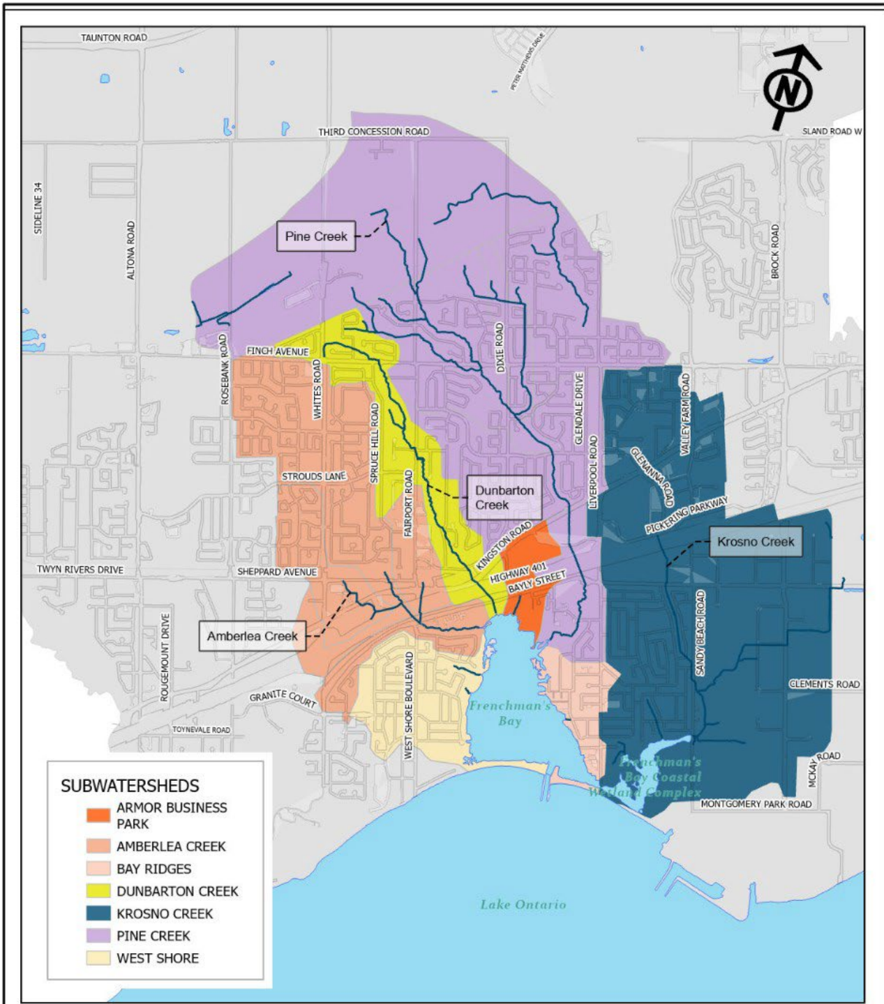
LOCATION MAP Frenchman's Bay Watersheds Study Area
