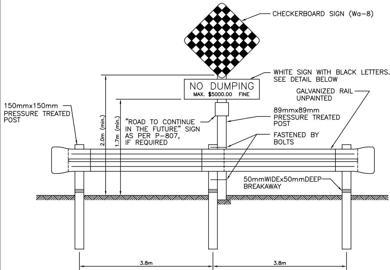
BARRICADE DETAIL
