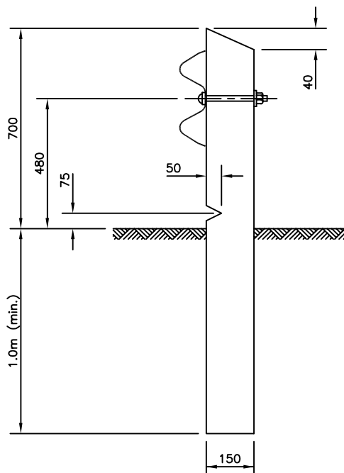
POST DETAIL
