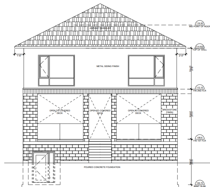
South – Rear Elevation
