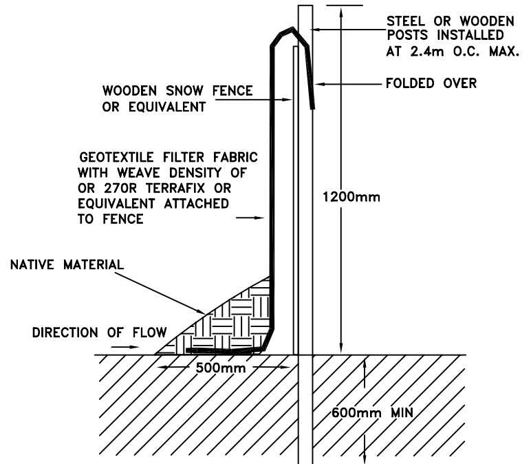
SECTION A-A FROZEN CONDITION
