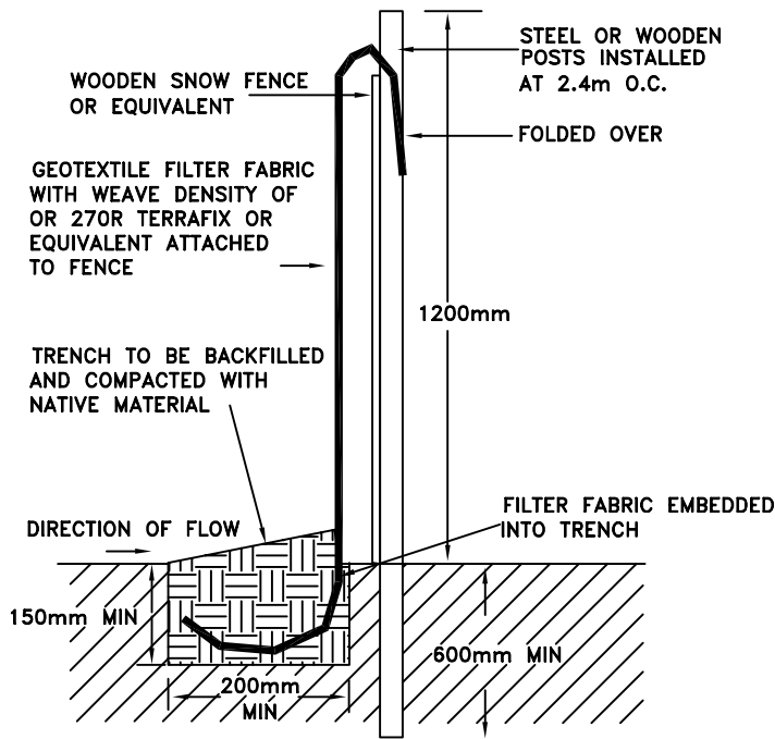
SECTION A-A NORMAL CONDITION
