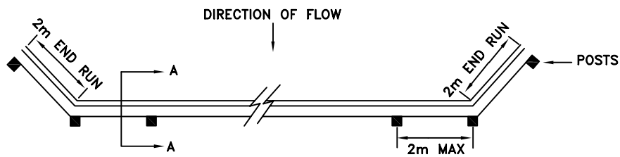
PLAN VIEW
